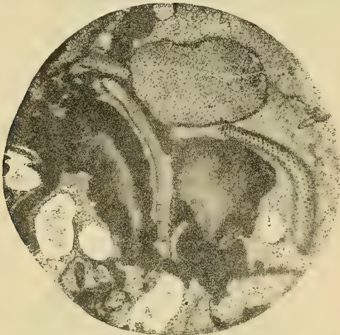
FIG. 8.—MICRO-PHOTOGRAPH OF A SECTION OF FOREST MARBLE. ( \times 22 diams.)
